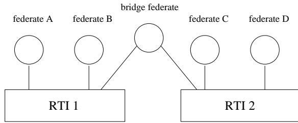
Figure 5: Interfederation architecture
