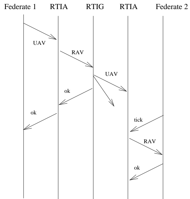
Figure 2: Data transfer scenario
