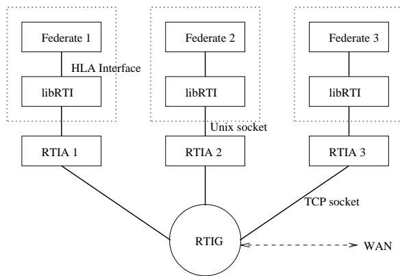
Figure 1: CERTI architecture
